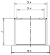
BS. High base plate
