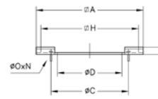
PA. Adaptation plate to mount accessories on roof fans
