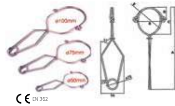
CE EN 362 LX06 Pipeform Anchor Stainless Steel Wire Size: 2" / 3" / 4" MBL: 27kn
