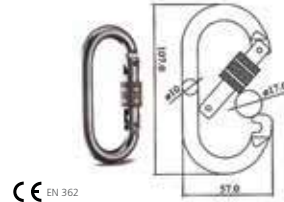
CE EN 362 LX03 Carabiner/ Screw Gate Alloy Steel. MBL: 22kn
