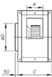
Supply on demand horizontal outlet (H) LG-90
