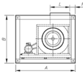
Supply on demand vertical outlet (V) LG-0
