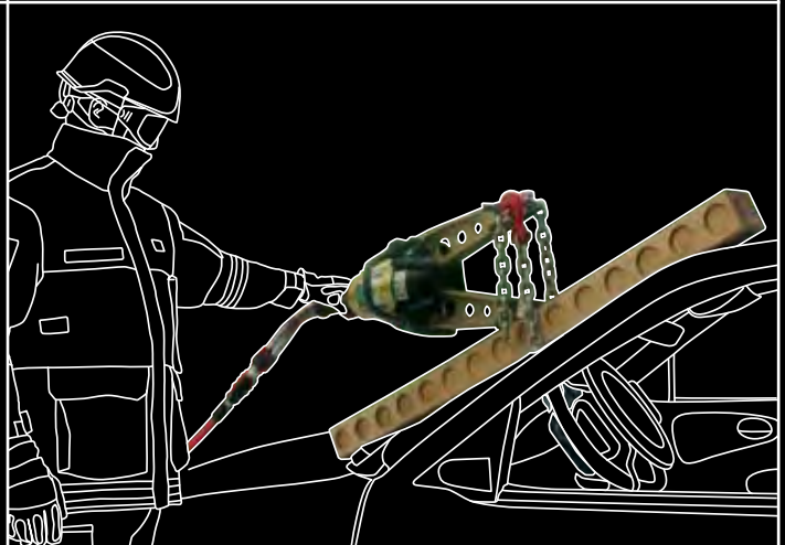
Apply spreader and pull steering wheel upwards
